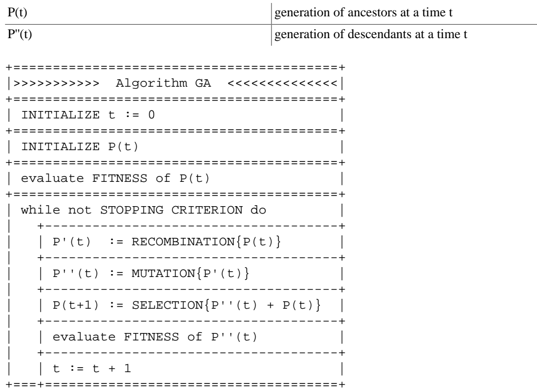
Figure 59.1. Structured Diagram of a Genetic Algorithm
